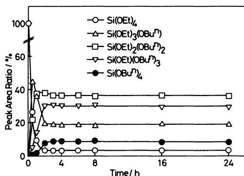
Fig. 6. Variation in the distribution of alkoxysilane species in the TEOS-BuOH solution at the BuOH/TEOS ratio of 4.0 with time of Amberlyst treatment at 40 °C.
