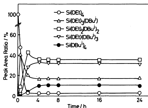
Fig. 7. Variation in the distribution of alkoxysilane species in the TEOS-BuOH solution at the BuOH/TEOS ratio of 4.0 with time of Amberlyst treatment at 40 °C.
