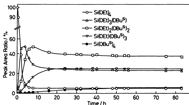
Fig. 8. Variation in the distribution of alkoxysilane species in the TEOS-BuOH solution at the BuOH/TEOS ratio of 4.0 with time of Amberlyst treatment at 40 °C.
